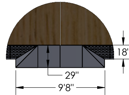
DETAIL C SCALE 1 : 75
